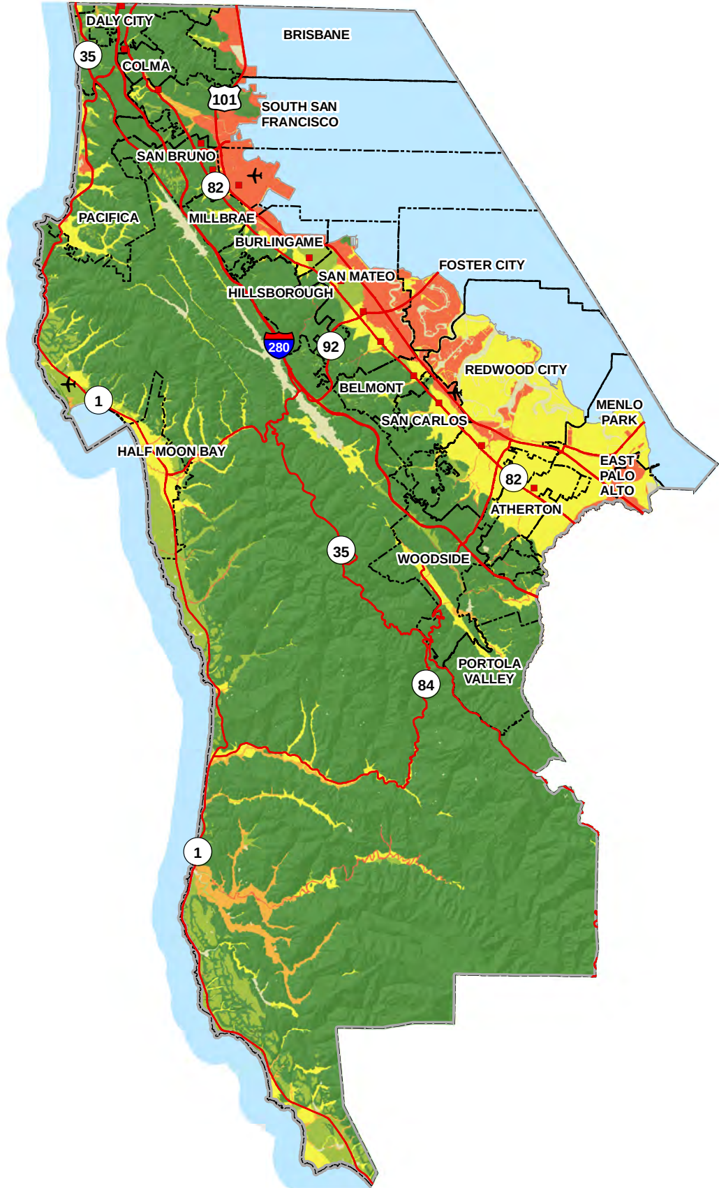
Figure 10-4. Liquefaction Susceptibility
